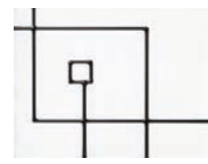
matrix
