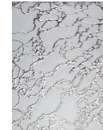
glacier
